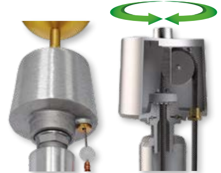
Internal Revolving - Spindle Design
