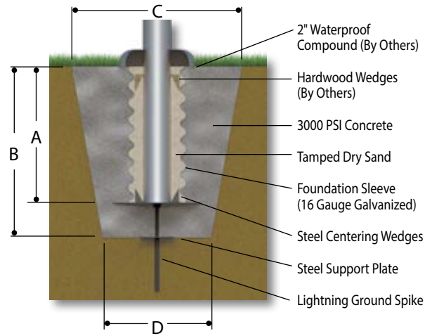
NAAMM's Metal Flagpole Manual offers basic suggestions on foundation measurements in firm, dry soil only using dry tamped sand and 3000 PSI concrete. Soil conditions vary by site. Exact foundation requirements should be verified by a Structural Engineer with knowledge of soil conditions in your locality.
