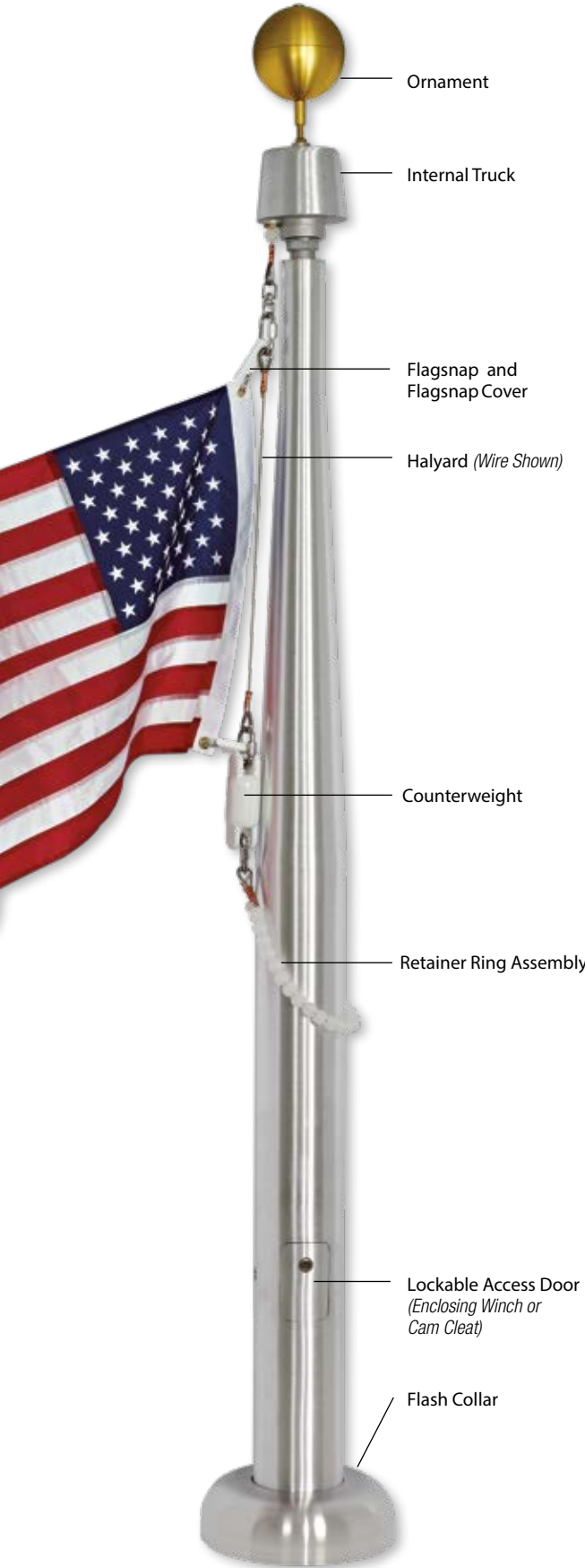
Wire Halyard
